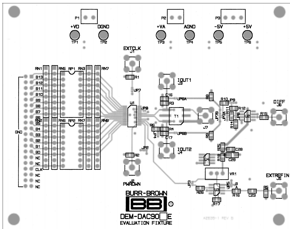
FIGURE 9. Top Layer (component side) with Silk-Screen (E-board).
