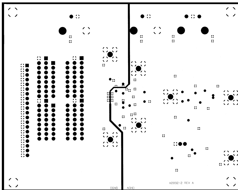
FIGURE 7. Ground Plane (U-board).
