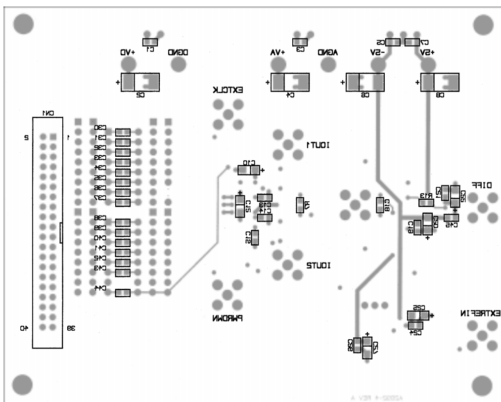
FIGURE 8. Bottom Layer with Silk-Screen (U-board).
