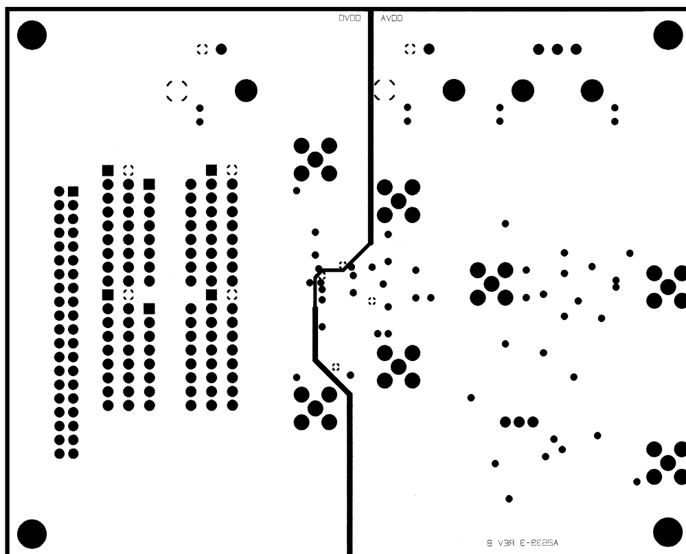
FIGURE 10. Power Plane (E-board).
